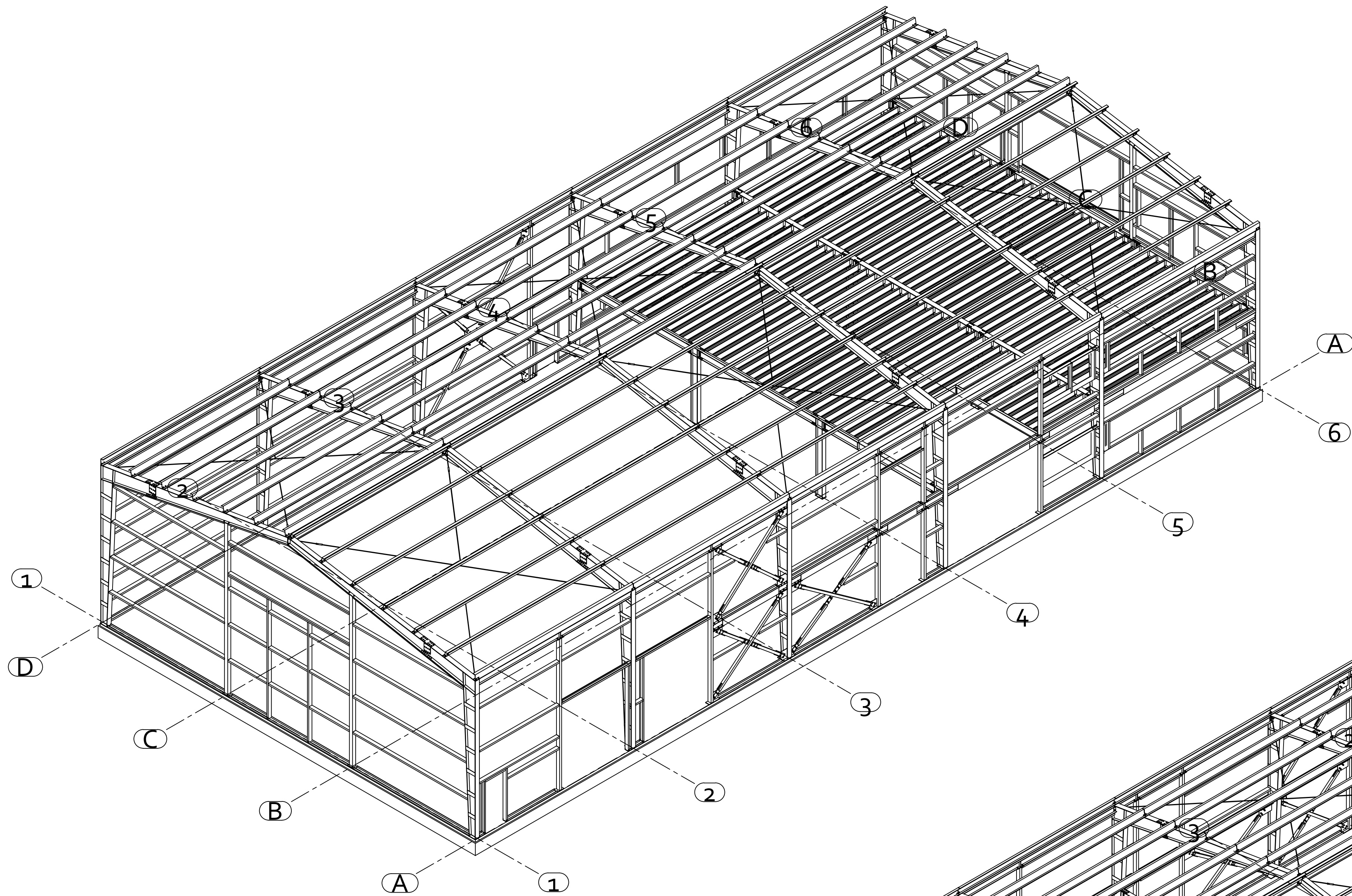
Isometric view South East
