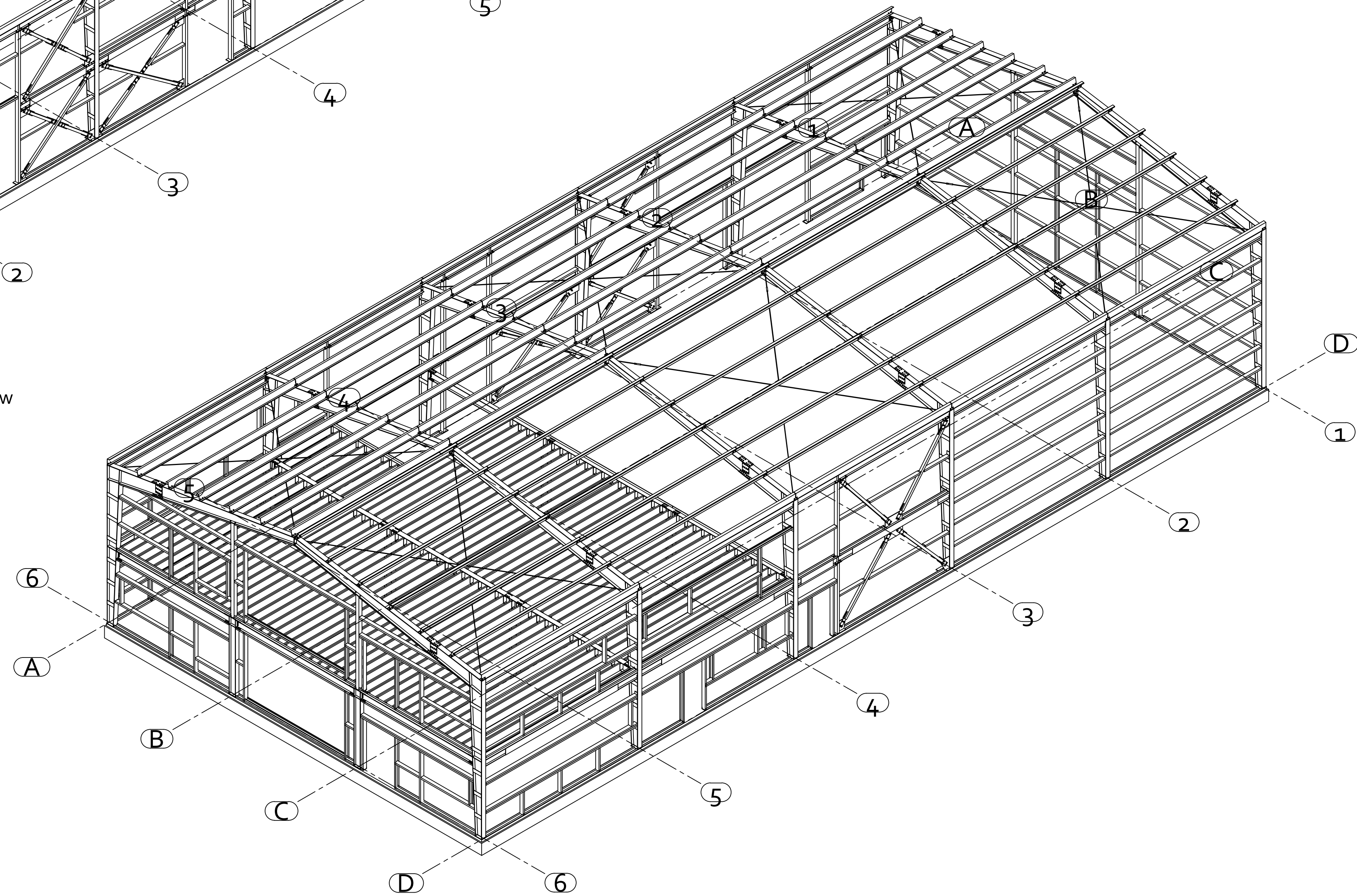
Isometric view North West
