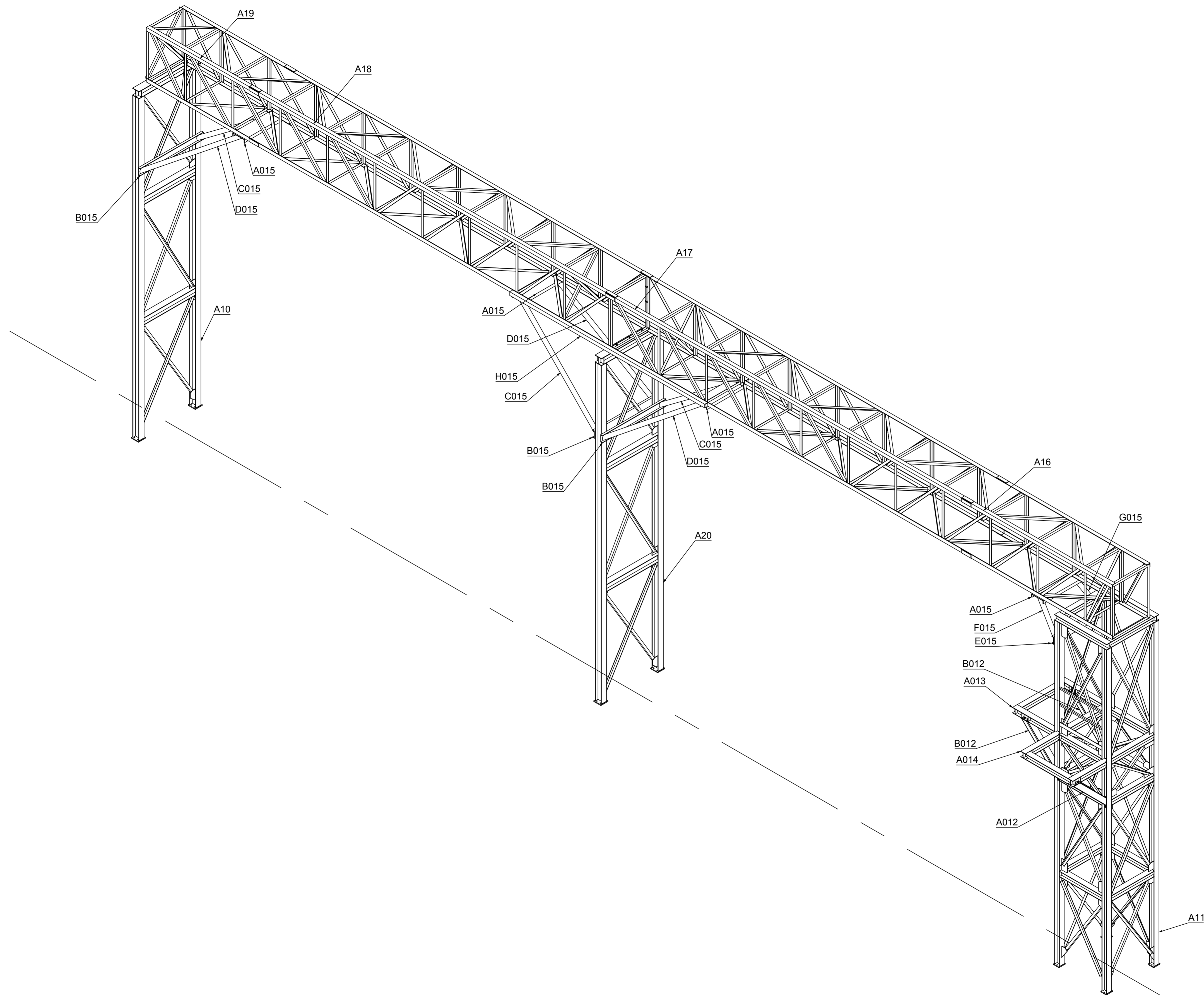
Isometric view
