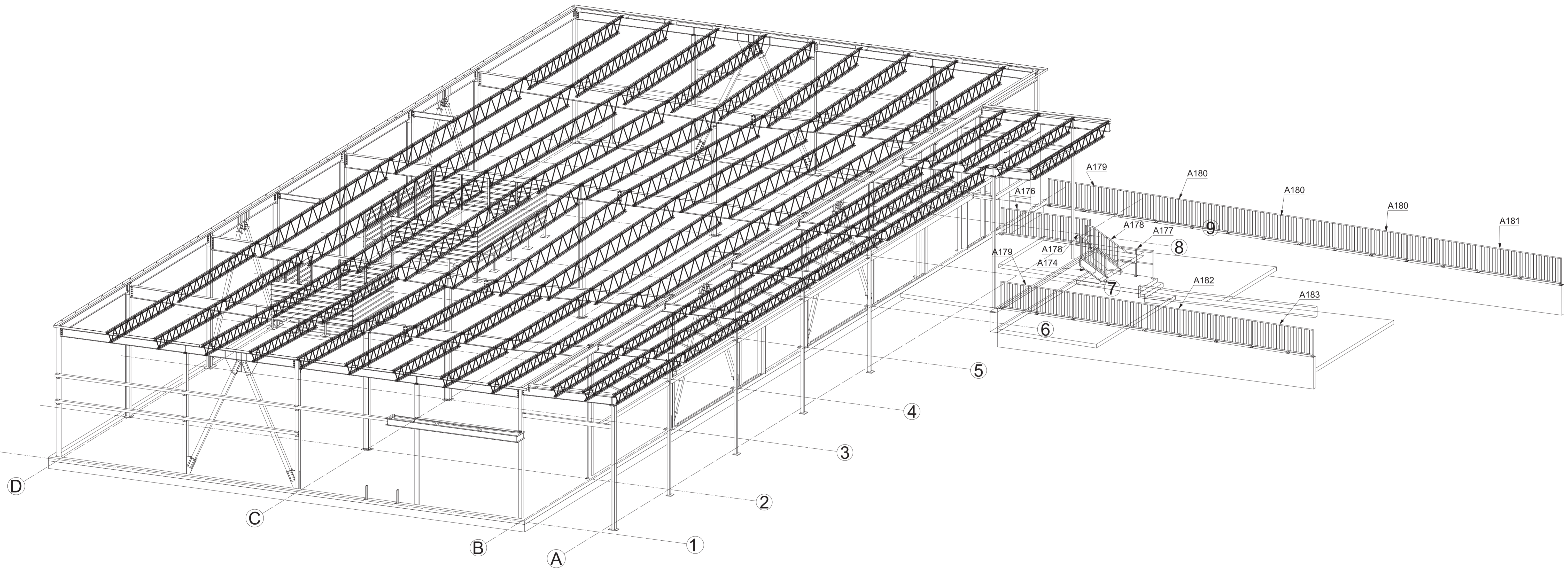
Isometric view
