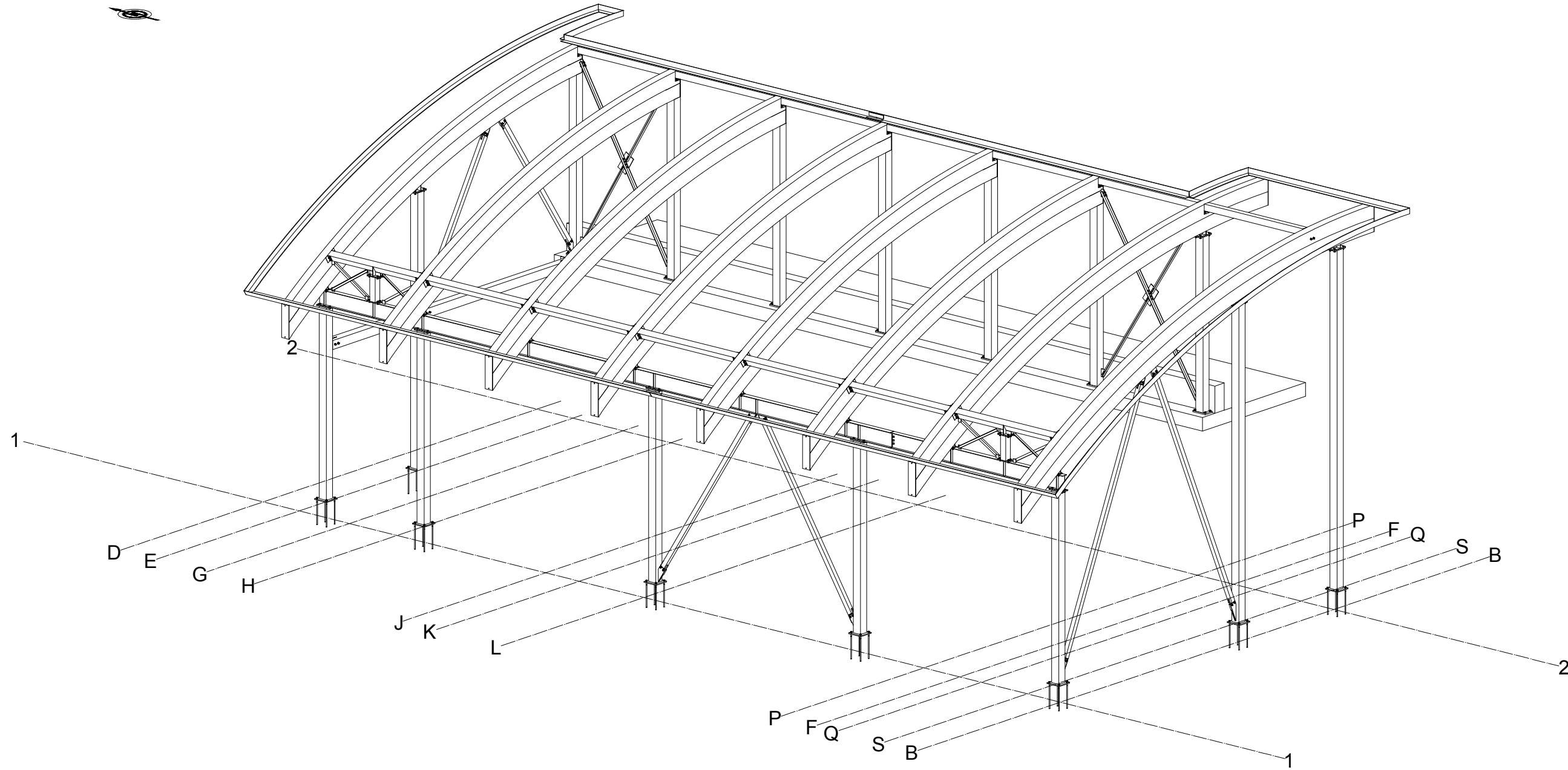
POOL ROOF ISOMETRIC VIEW
